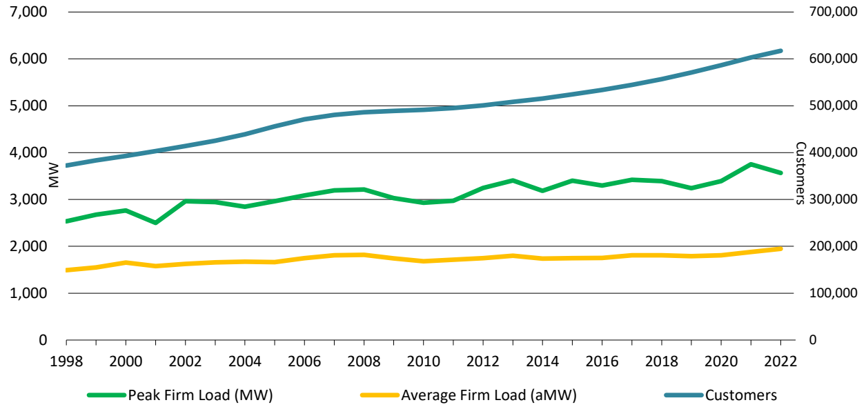
Figure 4.1 Historical load and customer data
