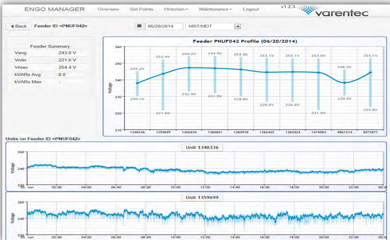
Figure 2. Baseline Voltage Sample
