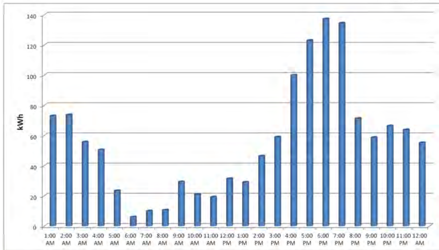
Figure 1. Charging times
