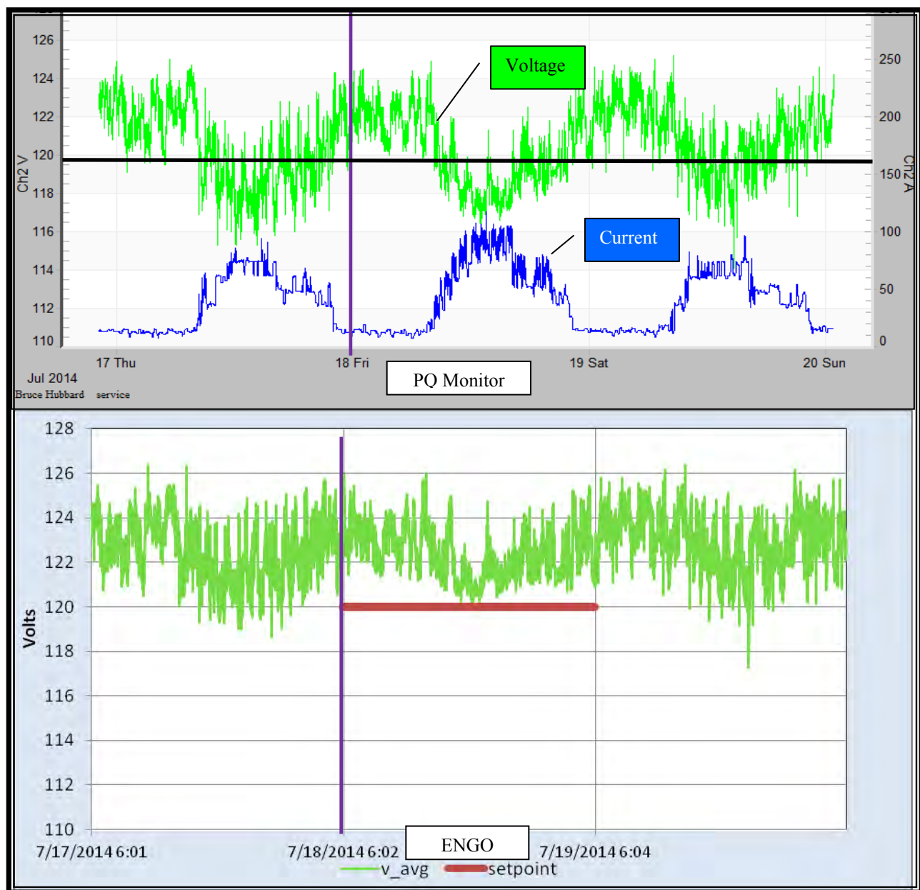
Figure 12. Average RMS Voltage at Unit #1360918
