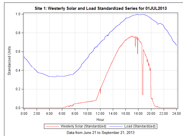
Figure 1. Southerly solar and load, 7-1-2013
