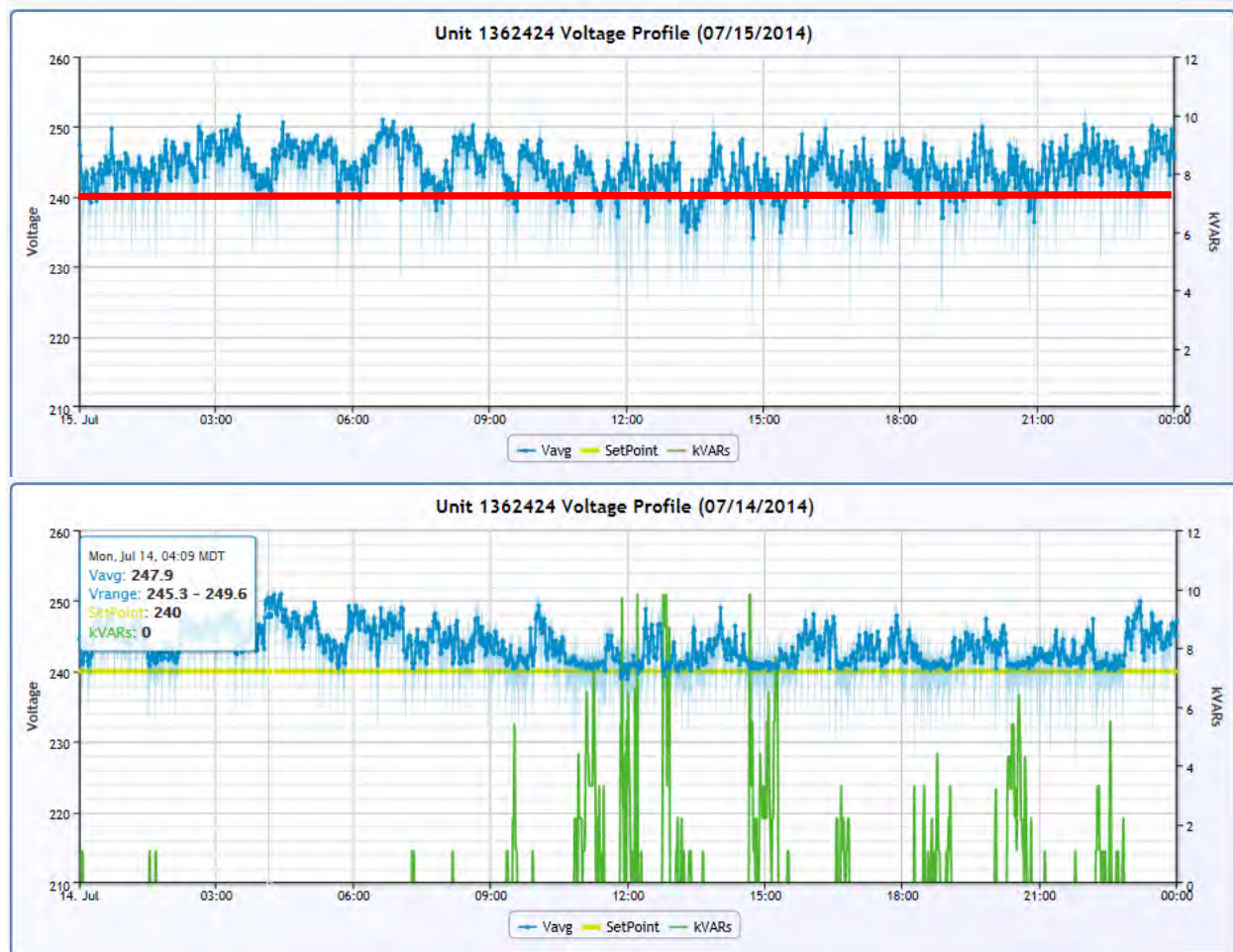
Figure 5. Unit 1362424 cycling
