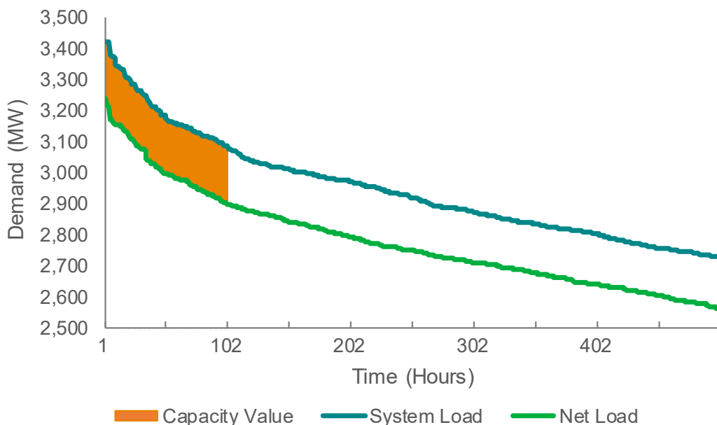
Figure 4.1 Capacity value of solar PV
